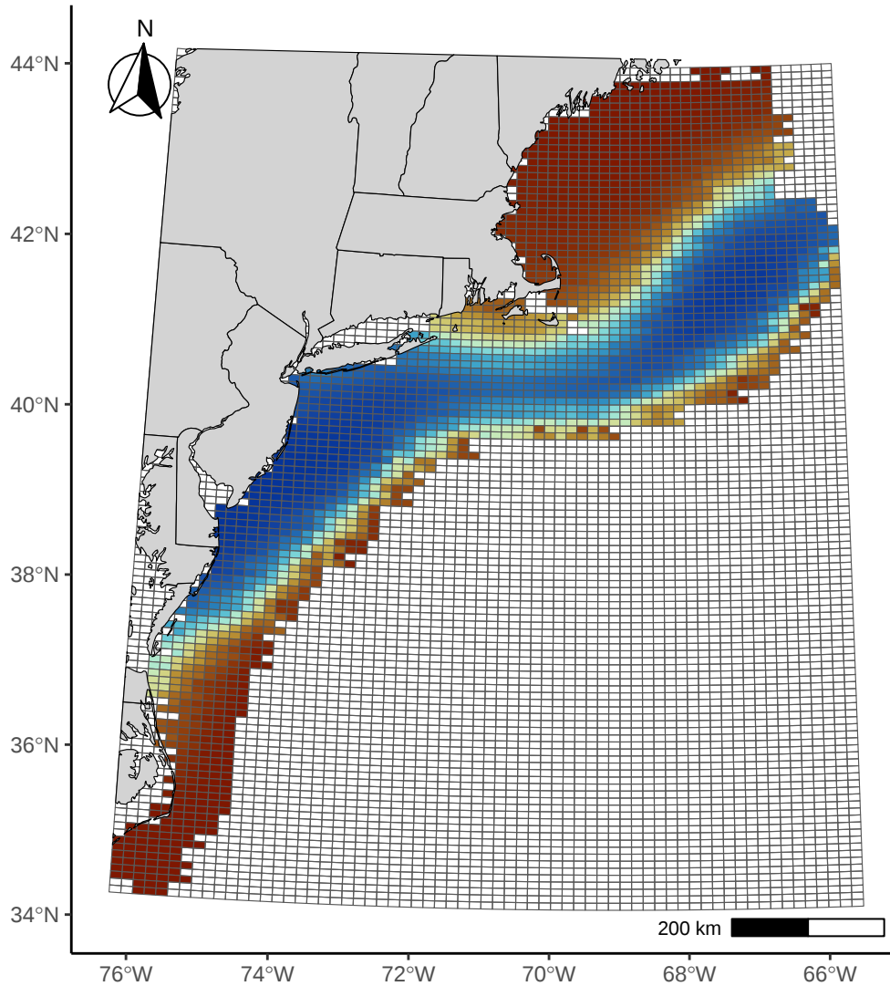
December 13–19, 2025: Atlantic Herring * (1–River Herring)
